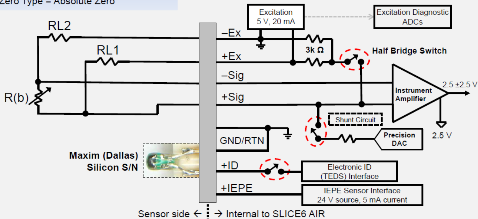
RTD (4-wire)
