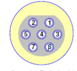
Omnetics 7-pin (male) MCP-7-SS (Rear View)
