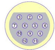
Omnetics MCP-12 (rear view)
