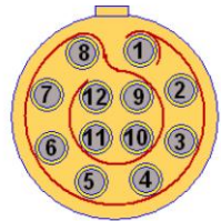
12-pin LEMO (F) rear view
