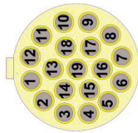
19-pin LEMO (M) rear view
