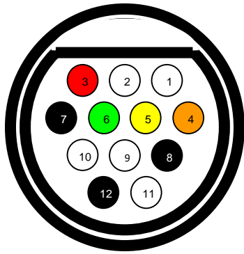
Omnetics MCP-12 rear view
