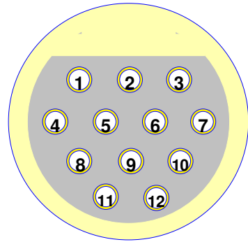
Omnetics 12-pin (sockets) MCS-12-SS
