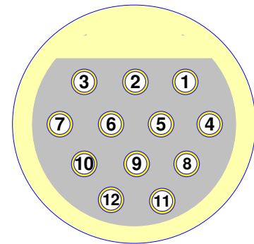
Omnetics 12-pin (pins) MCP-12-SS (Rear View)
