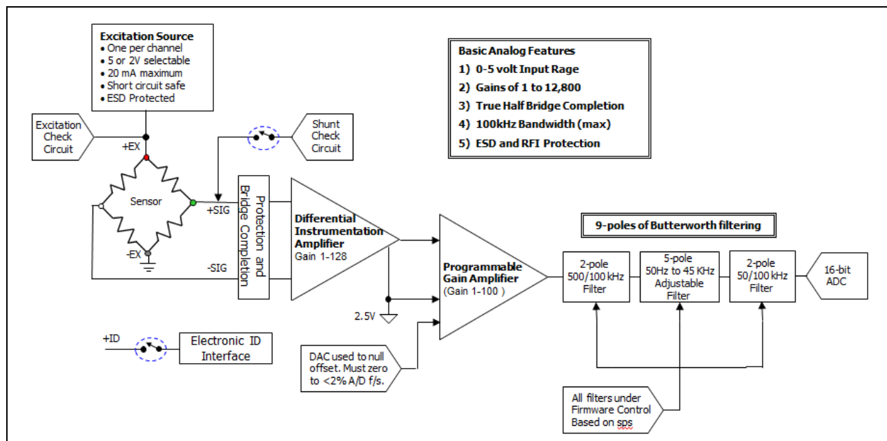
SLICE PRO SIM Single Channel Block Diagram
